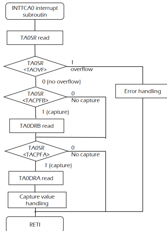
Interrupt process for double-edge capture
